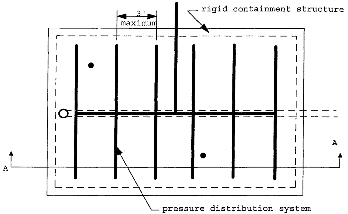
PLAN LAYOUT
